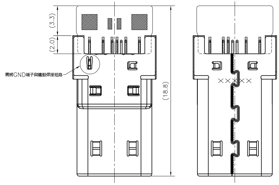
PADDLE CARD ASSEMBLY DIMENSIONS (REF.)
